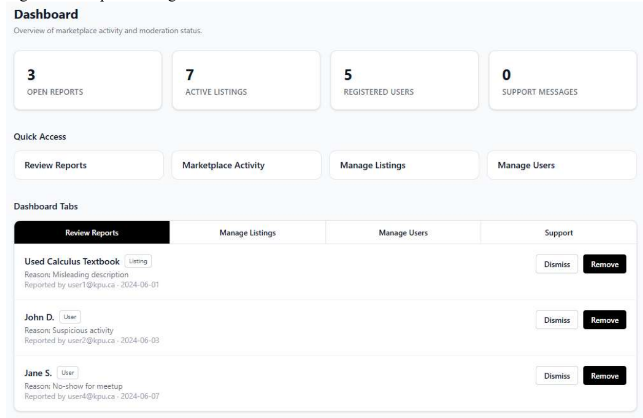
Figure 5.9: Report Management Form
